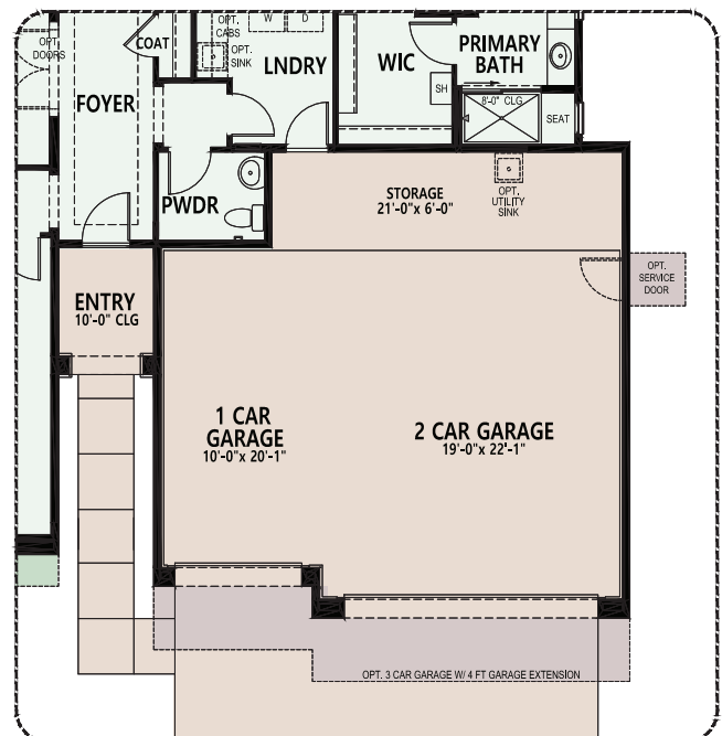
Opt. 3 Car Garage
